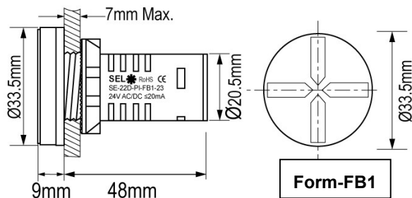
Outline Dimension
