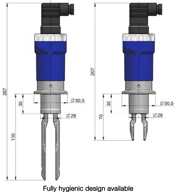
LD60 / LD61 - CLAMP ISO 2852 connection
