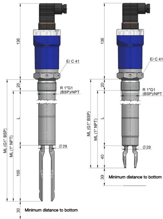
LD60ML / LD61ML (standard length \pm 1.5 mm)
