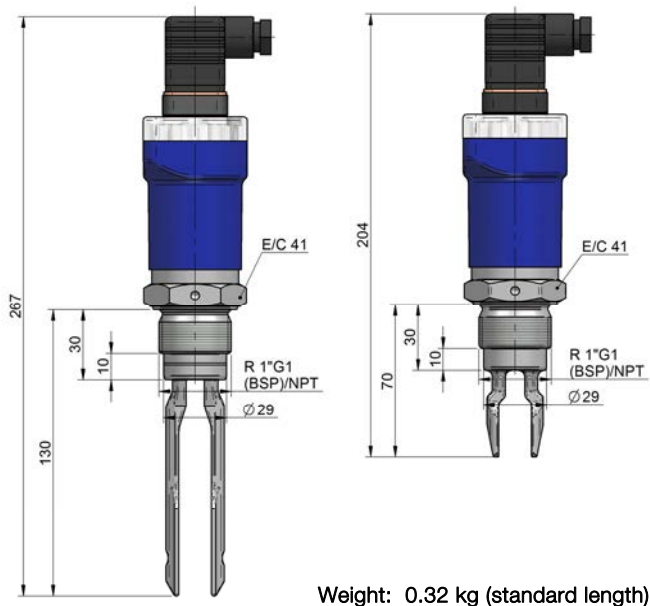
LD60 / LD61 - BSP / NPT threaded connections
