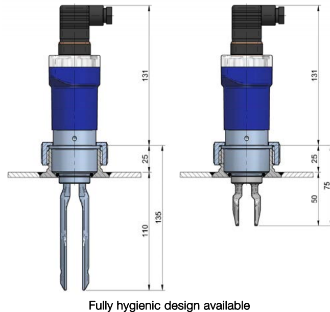
LD60 / LD61 - TF DIN405 flush mounting
