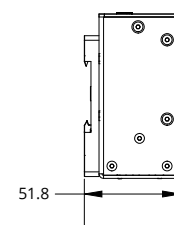
Dimension with DIN rail mount clips (on rear of Master 810 or 2410)
