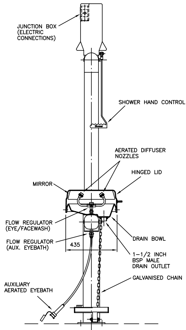
FRONT VIEW
