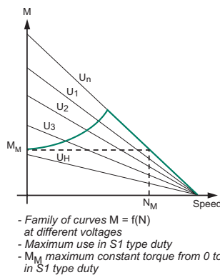
Characteristic curves of a high-torque motor
