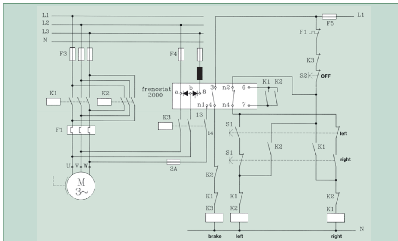
Circuit diagram 2
