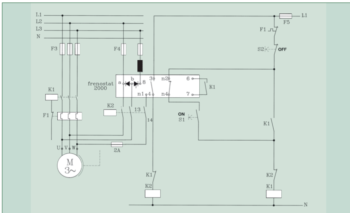
Circuit diagram 2
