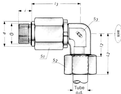
Male stud elbow rotary fittings: DG 104/--PSR
