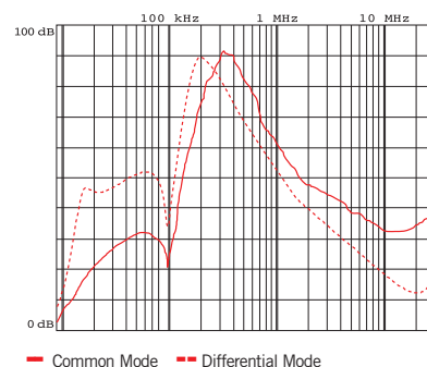
Typical attenuation 500A – 3000A
