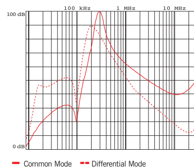
Typical attenuation 5A – 400A
