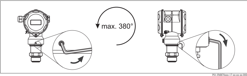
Align the housing by loosening the Allen screw. Aluminum housing (T14 and T15): 2 mm Allen key; Stainless steel housing (T17): 3 mm Allen key
