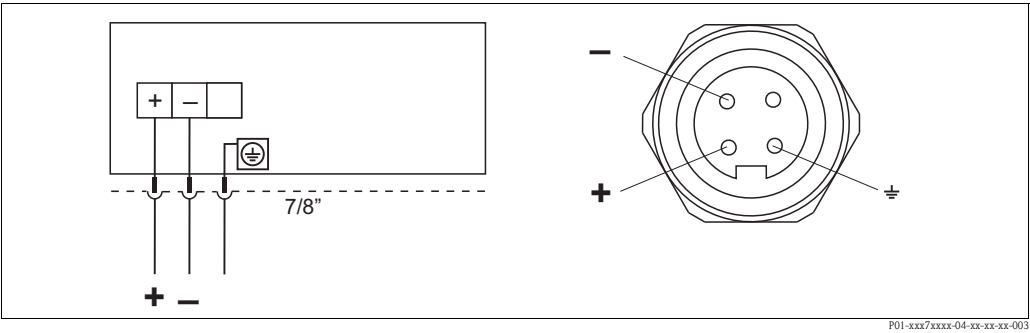
Left: electrical connection for devices with a 7/8" connector Right: view of the connector at the device
