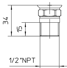
1/2"NPT
