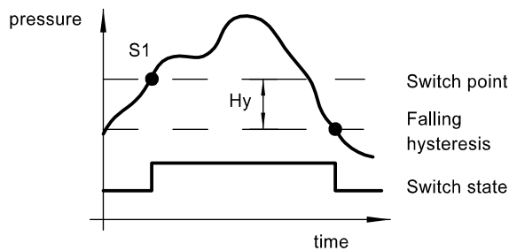
-falling hysteresis-
