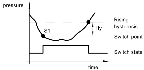
-rising hysteresis-
