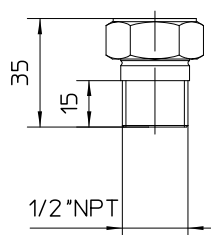
1/2"NPT
