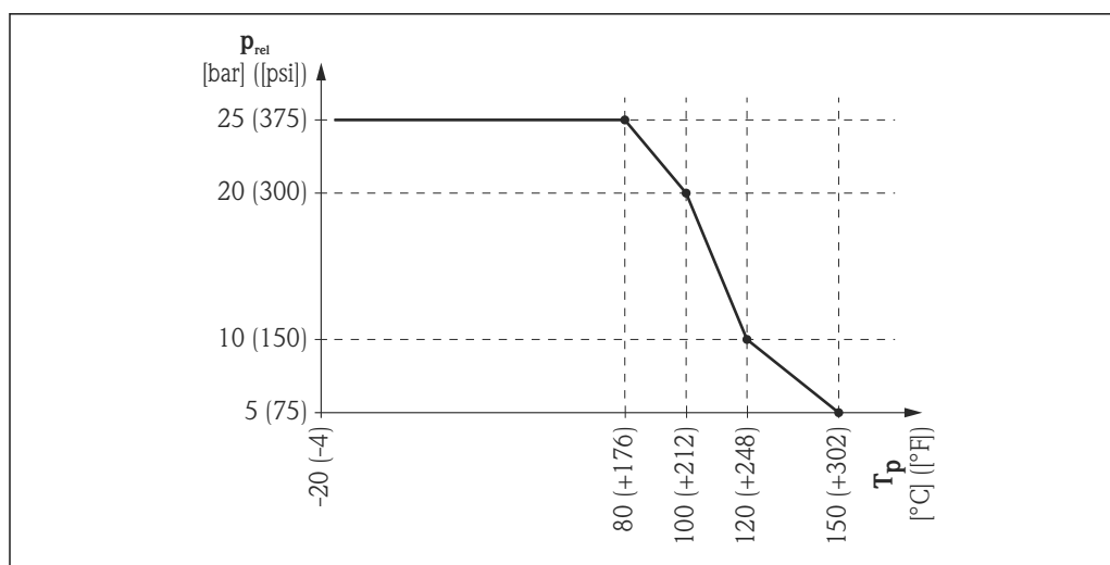
17 FMR54 with planar antenna: Admissible range of process temperature and process pressure
