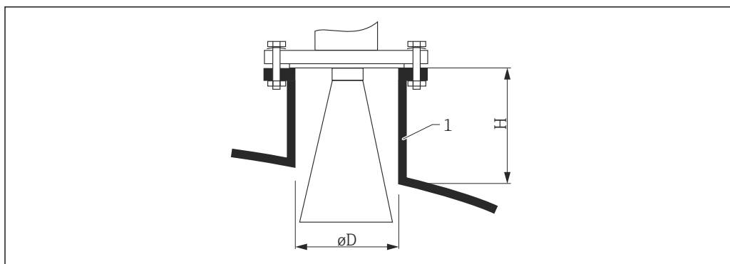
12 Nozzle height and diameter for the horn antenna (FMR54)
