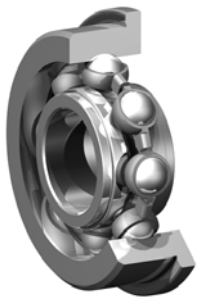
Ribbon Cage
