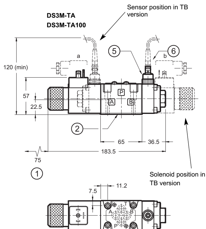
MOUNTING SURFACE ISO 4401-03-02-0-05 (CETOP 4.2-4-03-350)
