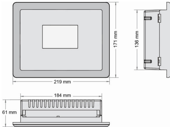
easYgen-2200/2300
