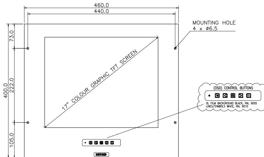
FRONT VIEW
