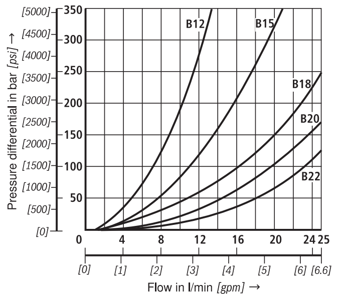
\Delta p - q_v characteristic curves
