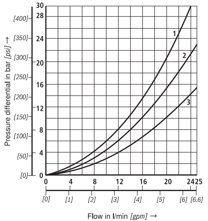
\Delta p - q_v characteristic curves
