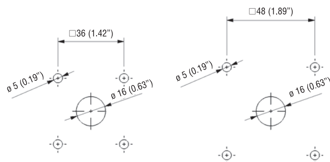
Four-screws fixing
