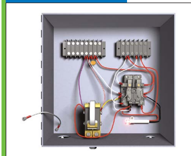
Figure 2: 3539 Controller
