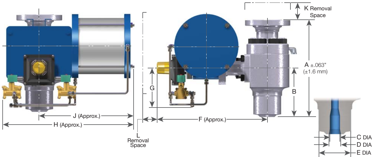
3537, 3538 & 3547W w/ LEDEEN GS620 & GS628 Actuators
