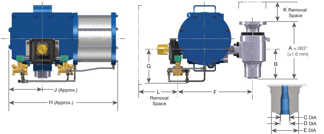
Optional Accessories General Dimensions (Buttweld)
