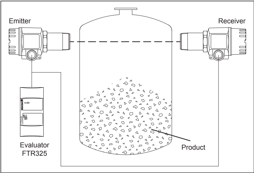
Example 2: Limit detection of bulk solids
